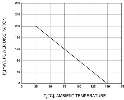
Figure 3. Power Derating
